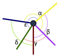
Figure 5: Angle criterion: \gamma < \beta < \delta < \epsilon < \alpha .
