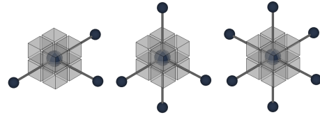
Figure 11: Examples of orthogonal intersections.
