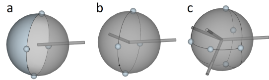
Figure 1: Quad partitions of a sphere around vertices of degree 1, 2, and 4.
