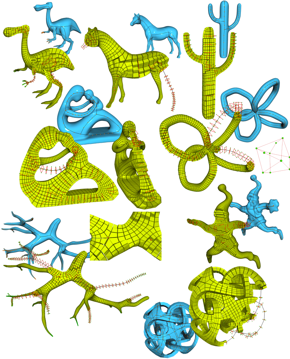
Figure 18: Some meshes obtained with our method. The skeleton (black) extracted from the surface mesh (blue) and connection surfaces (red) are displayed along with the hexahedral cells (yellow). Quality measures for these meshes are indicated in Table 1. From top-left to bottom-right: Dinopet, Horse, Cactus, Fertility, Cycles, Vessel, Santa and Metatron.
