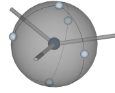
Figure 10: "Orange slice" handling of a flat branching point of degree 3.
