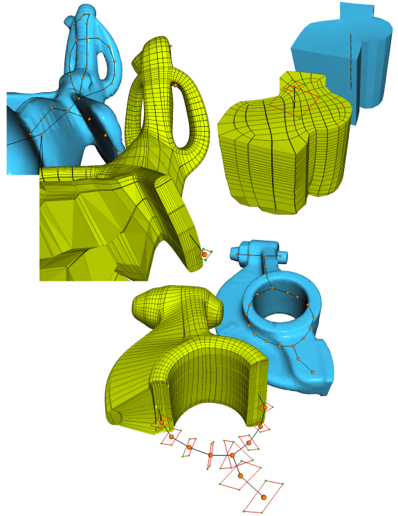
Figure 17: Shapes that will typically be poorly reconstructed with our method, as the radial nature of the generated structure is not able to capture the flat areas or complex cross section. Top: Elephant and Mechanical piece. Bottom: Rocker arm.
