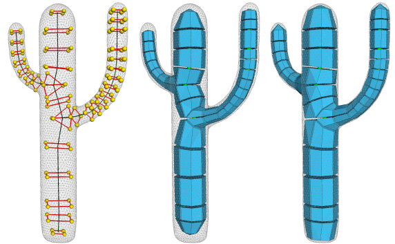
Figure 14: Generation of the connection surfaces and rough volume mesh
