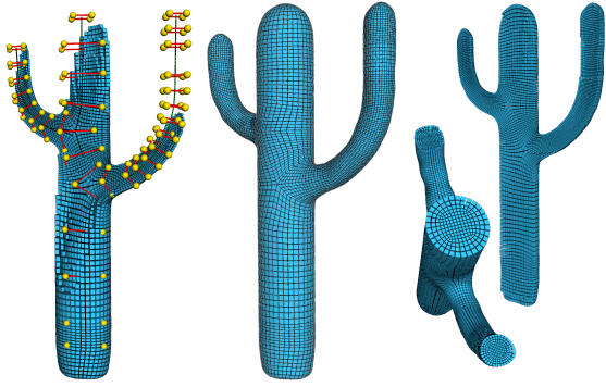
Figure 15: Refinement and geometry optimization
