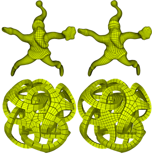
Figure 16: On the left, results obtained by (Livesu et al., 2016) (Santa) and (Livesu et al., 2020) (Metatron), on the right, our results. Combining cube fitting and sphere partitioning techniques depending on the angles in the branching points improves the symmetry and the overall elements quality of the obtained hexahedral meshes.
