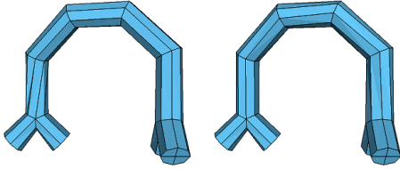
Figure 2: Twist redistribution between two branching points.
