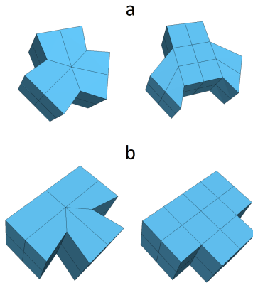
Figure 12: Comparison of sphere partitioning and cube insertion technique on two degree 3 vertices. Minimum scaled Jacobian: a) 0.802 (left) 0.409 (right); b) 0.533 (left) 1 (right).
