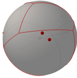
Figure 9: A failure example of the quad partitioning of the sphere: not all quads contain their respective point.
