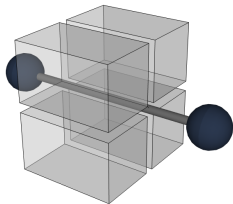
Figure 3: Hexahedra chunk around an edge of the skeleton.
