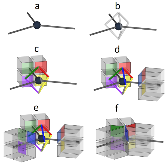
Figure 4: The connection surface built on each skeleton vertex is used as a scaffold for the geometry and connectivity of the hexahedra. (a) a vertex incident to three branches (b) the connection surface composed of three quads (c,d,e) incident chunks are paired (indicated by colour) with their associated quad edges (f) pairs of hexahedra are connected.
