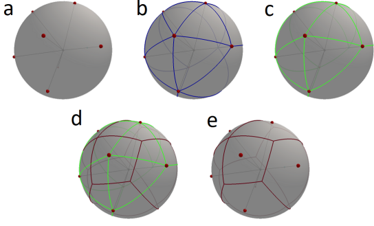
Figure 8: Quad partitioning algorithm on a sphere. Given an initial set of points, we obtain a quad mesh where each quad contains one of the given points. (a) Intersection of the branches with a sphere (b) Construction of the Delaunay triangulation (c) Remeshing of the triangulation (d) Construction of the dual mesh (e) Resulting quad mesh connection surface.
