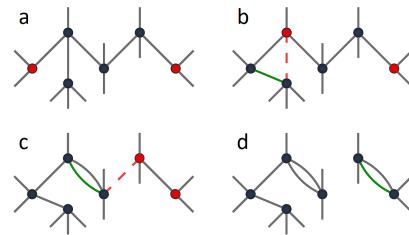
Figure 7: Connectivity modification between two vertices of degree 3 (in red) separated by an even length path (a). An adjacent vertex is used to shift a degree 3 vertex by one step along the path (b). Then we are left with the odd length case (c-d).
